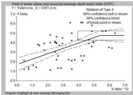
Figure 14. Segmented regression of the wheat yield ( Y ) on the average DWT value in winter on the X -axis. There is a breakpoint (BP) at X = 0.53 m that may be taken as the CDW value. This value corresponds to the breakpoint of the lower envelope determined in figure 13.
