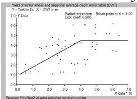
Figure 15. Partial regression of the wheat yield ( Y ) on the average DWT value in winter on the X -axis. There is a breakpoint (BP) at X = 0.4 m. Statistically, the maximum horizontal stretch ranges from X = 0.4 m until X = 0.65 m.
