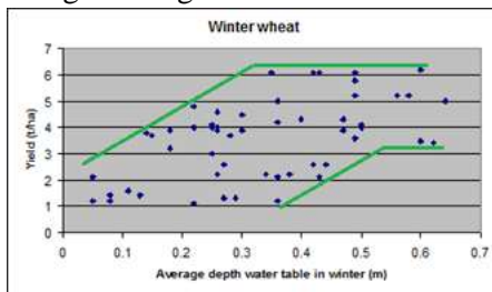
Figure 13. Yield (t/ha) of winter wheat on the Y-axis versus average value of DWT (m) in winter on the X-axis using the traditional envelopes method estimated by eye.
