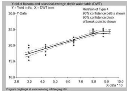
Figure 2. Segmented regression of the banana yield ( Y ) on the annual average DWT value on the X -axis. There is a breakpoint (BP) at X = 0.85 m that may be taken as the CDW value. The coefficient of explanation ( CE or R^2 ) equals 0.825. The values of BP and CE can be read from the output file of SegRegA (see Appendix C).
