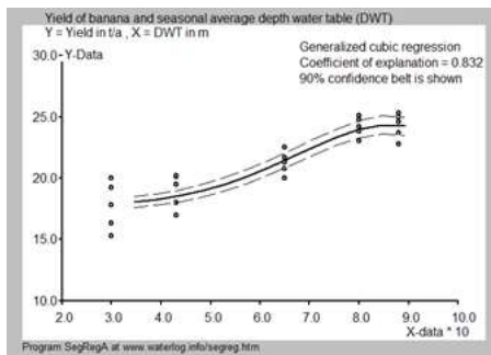
Figure 5. Generalized cubic regression of the banana yield (Y) on the yearly average annual DWT on the X-axis.
