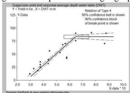
Figure 11. Segmented regression of the sugarcane yield
