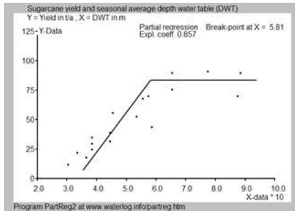
Figure 12. Partial regression of the sugarcane yield (Y) on the seasonal average DWT value on the X-axis. There is a breakpoint (BP) at X=0.58 m. Statistically, the maximum horizontal stretch ranges from X = 0.58 m until X = 0.9 m.
