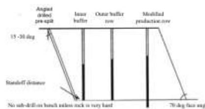
Typical pre-split design
