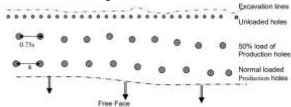
Line drilling along the final excavation
