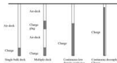
Pre-split loading options
