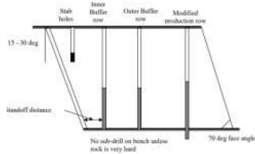
Pre-split design in unfavorable conditions
