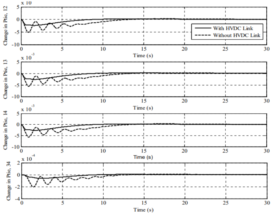
Fig 7: Tie line power deviations with \Delta P_{d1} = 0.01
